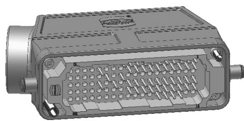
Figure 36 Metal Plug with 108 Pins
