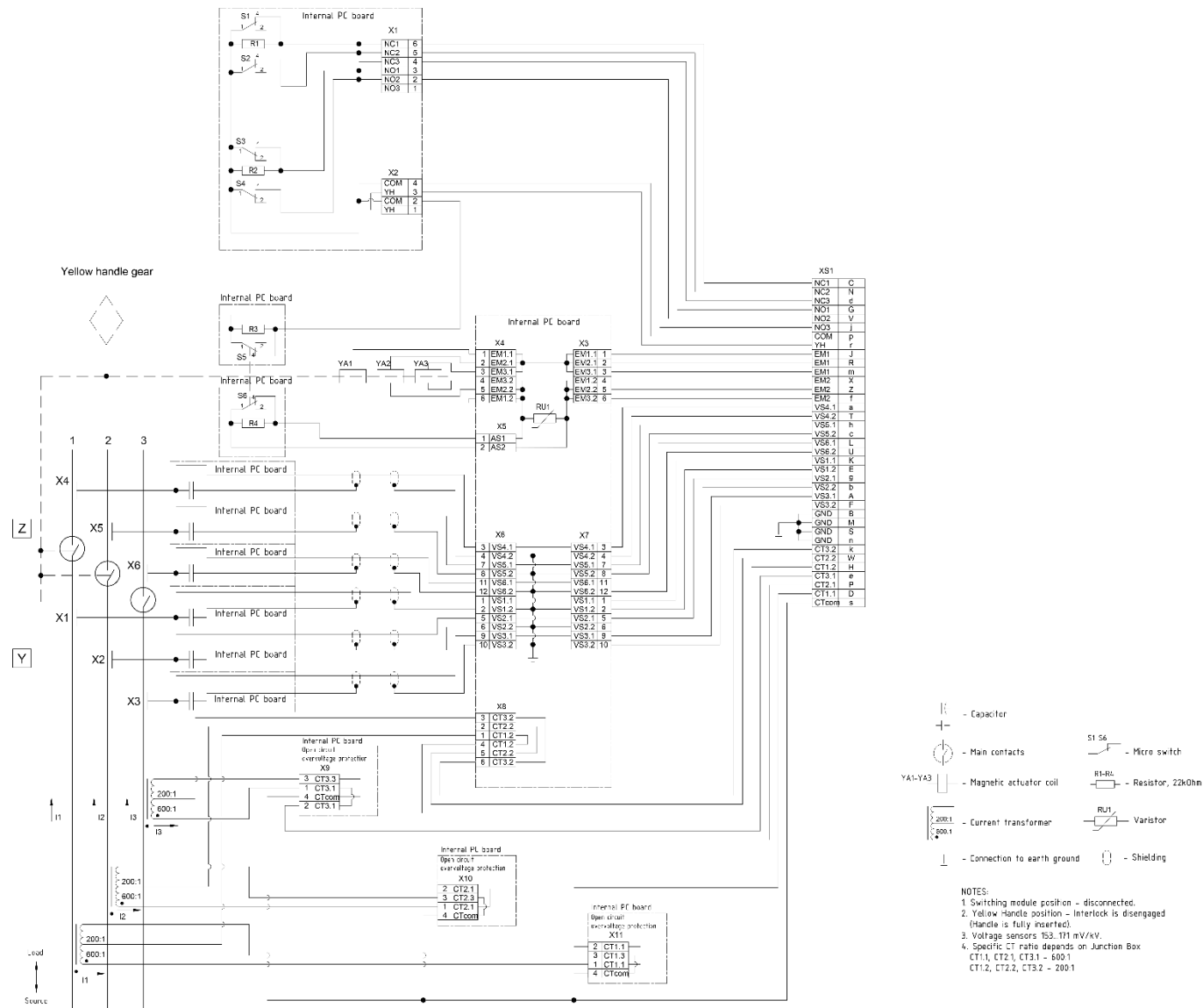
Figure 25 OSM35_Smart_5(600.200_150_AII) circuit diagram
