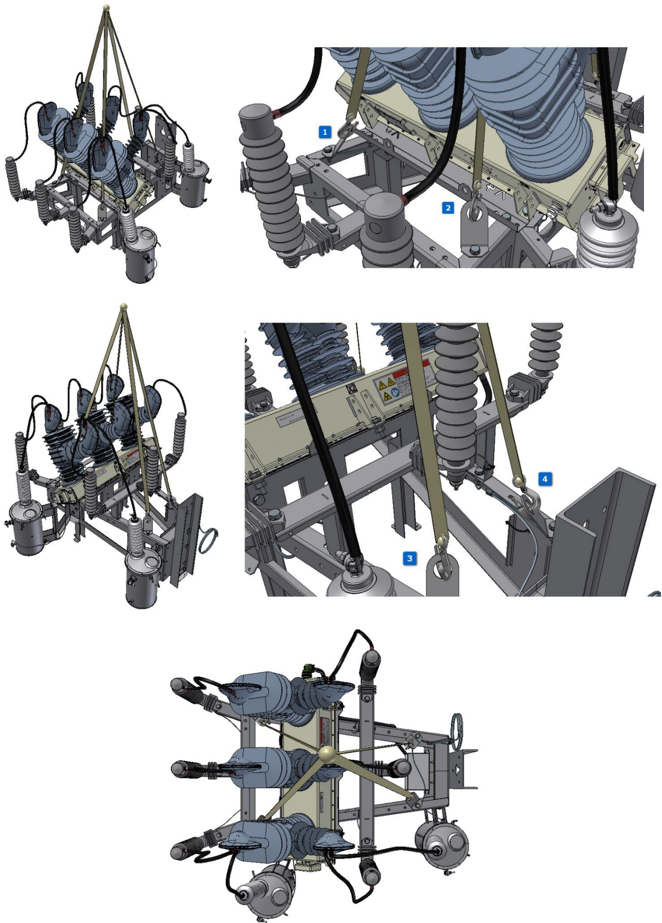
Figure 16 Lifting the recloser
