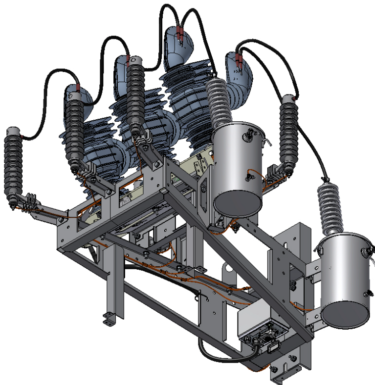
Figure 21 Rec35_Smart5_HDG earthing arrangement
