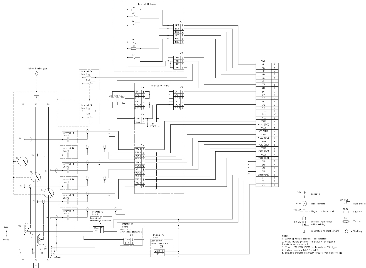
Figure 24 OSM35_Smart_5(AII_150_AII) circuit diagram
