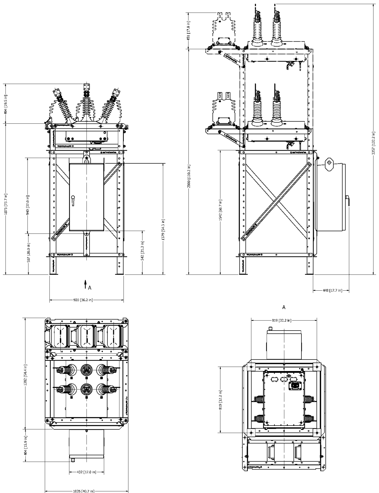
Figure 34 Stainless steel substation mounting kit
