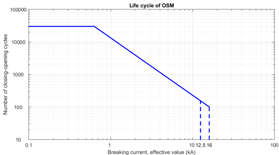
Figure 2 Outdoor Switching Module electrical endurance
