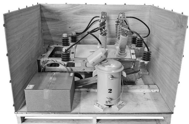
Figure 28 Packing carton
