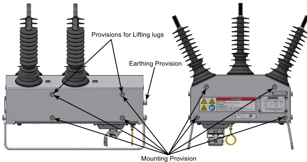
Figure 6 Threaded holes arrangement
