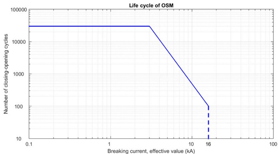
Figure 1 Outdoor Switching Module electrical endurance
