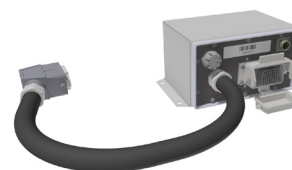
Junction box providing variable CT ratio for OSM25_AL_5 (600:1, 300:1, 200:1, 150:1, 100:1, 60:1) and safe trip functionality.
